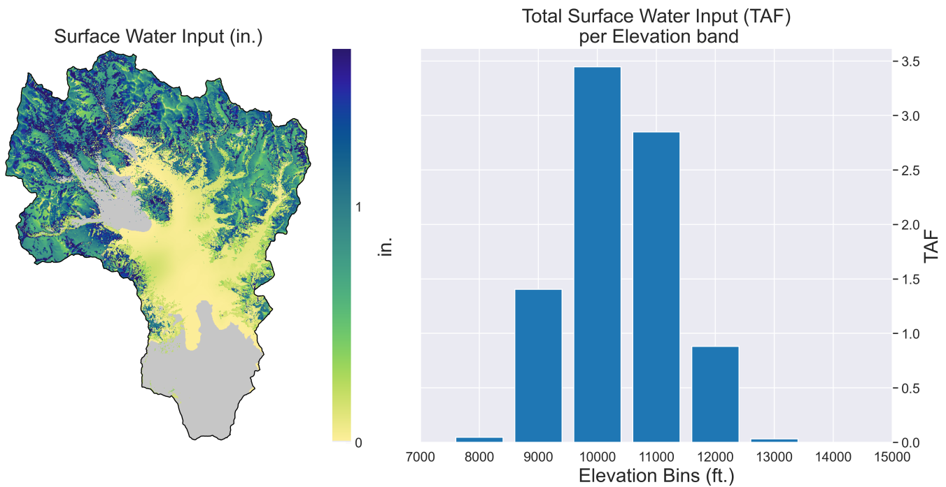
Fig.6 Accumulated Surface Water Input from 2023-05-22 to 2023-05-23
