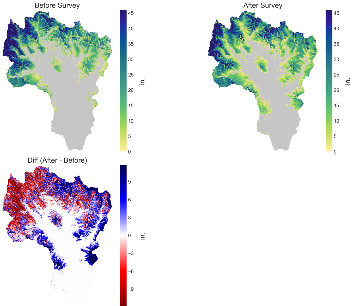
Fig.3 Change in Snow Water Equivalent from 2023-05-22 to 2023-05-23
