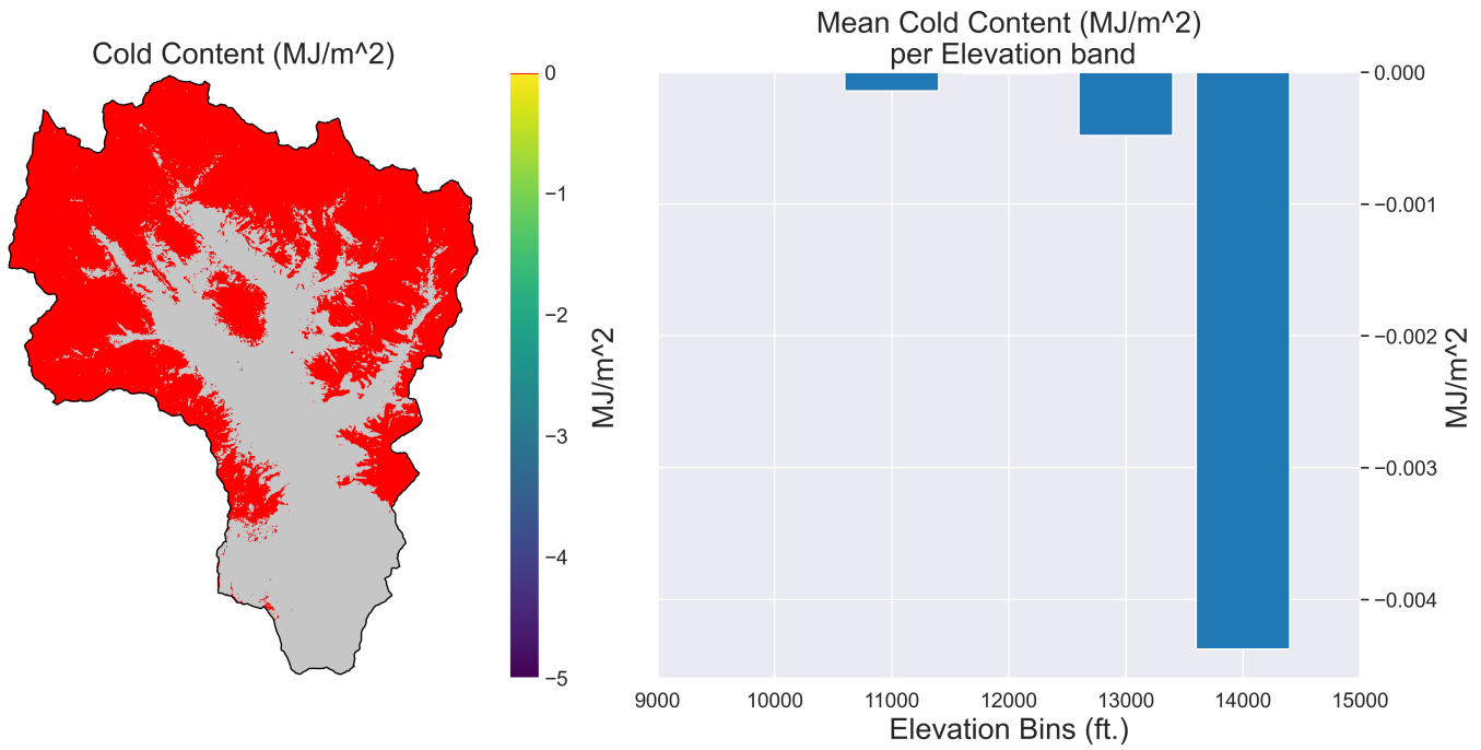
Fig.7 Cold Content as of 2023-05-23
