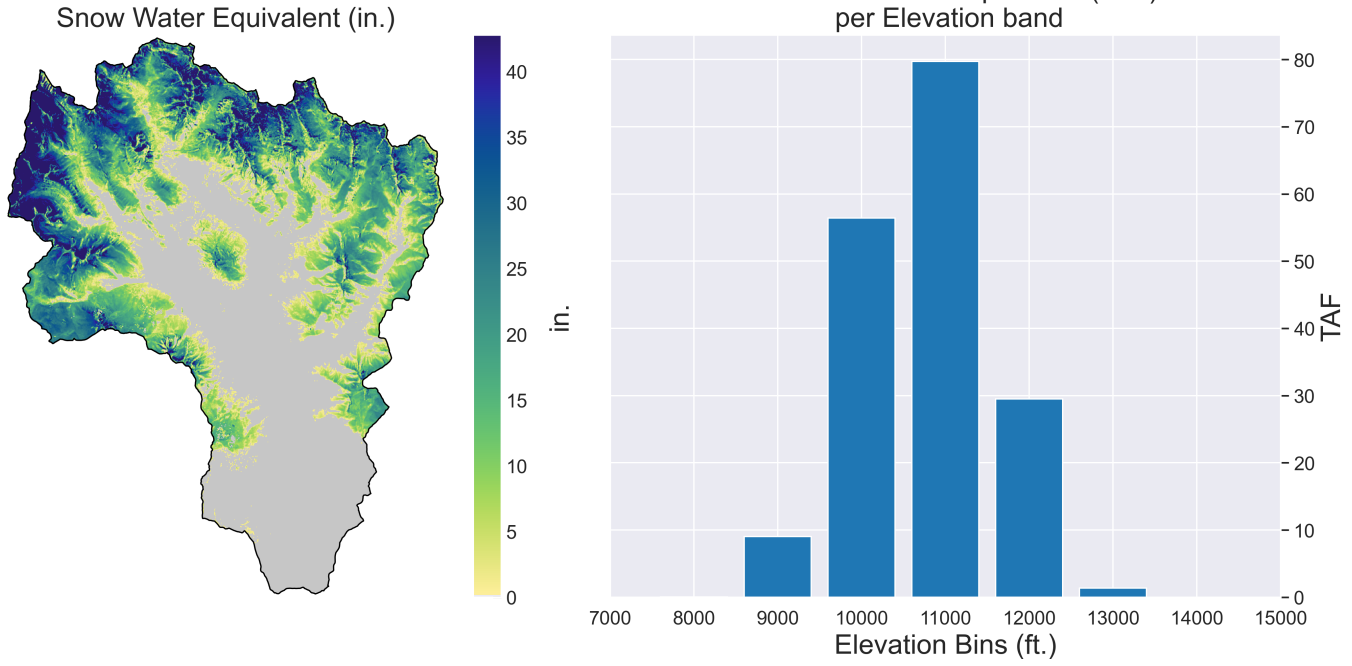
Fig.5 Snow Water Equivalent as of 2023-05-23
